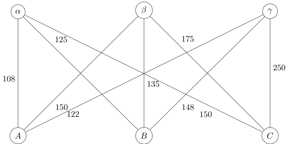
Figure 3.1: Bipartite graph
